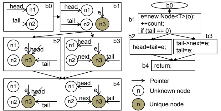
Fig. 6: Example connectivity graphs
