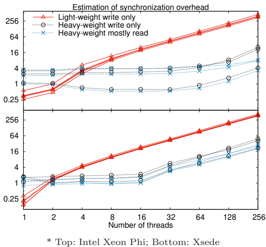
Fig. 9: Synchronization overhead of auto-generated code
