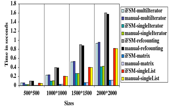
Figure 8: Performance using different input sizes
