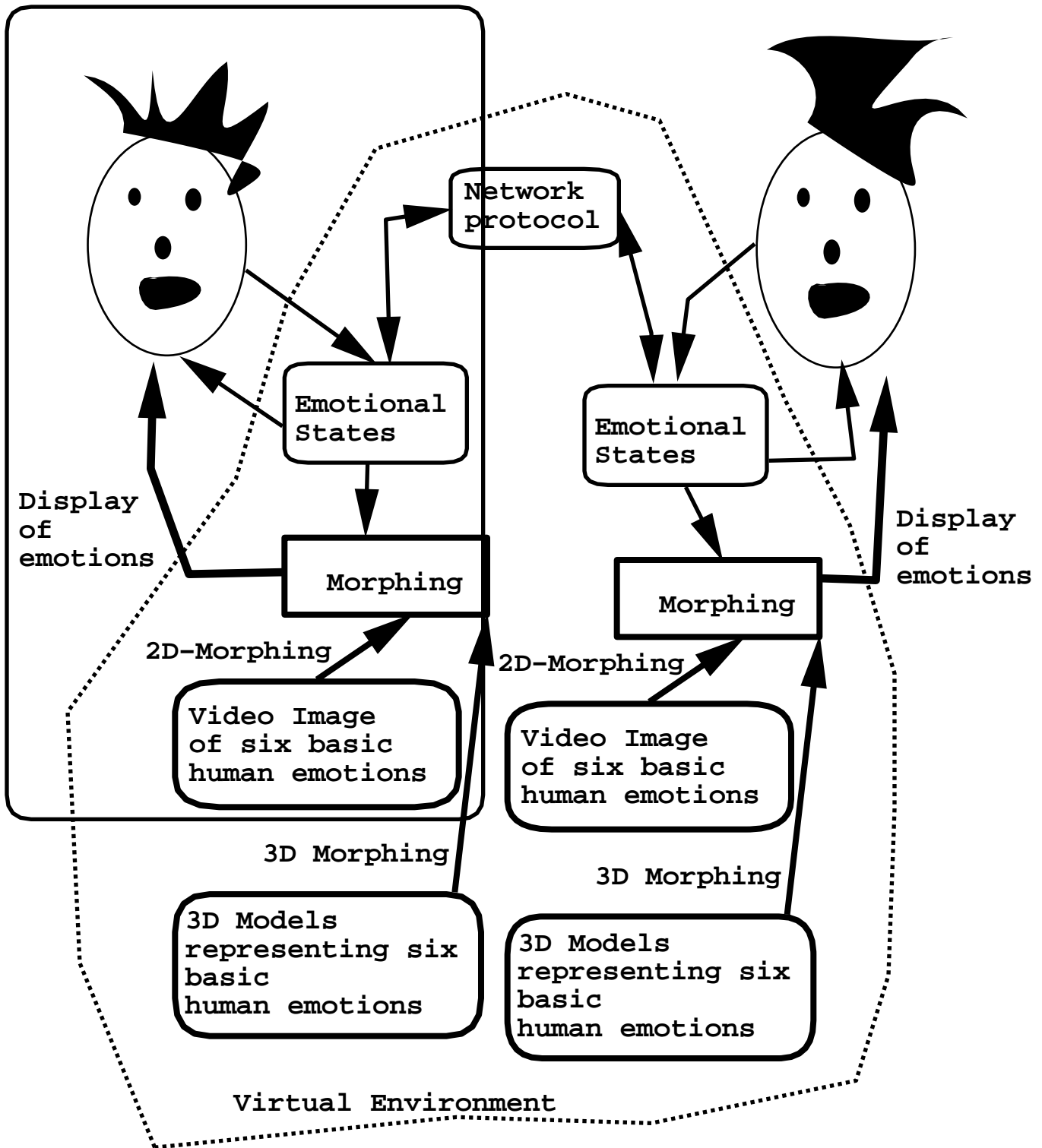
Modeling Emotions of multiple Avatars in a Virtual Environment for NonVerbal Communication
