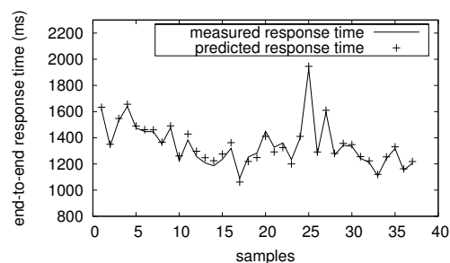
Fig. 4. APPLEware’s performance prediction (APP1) in the presence of interference effects.
